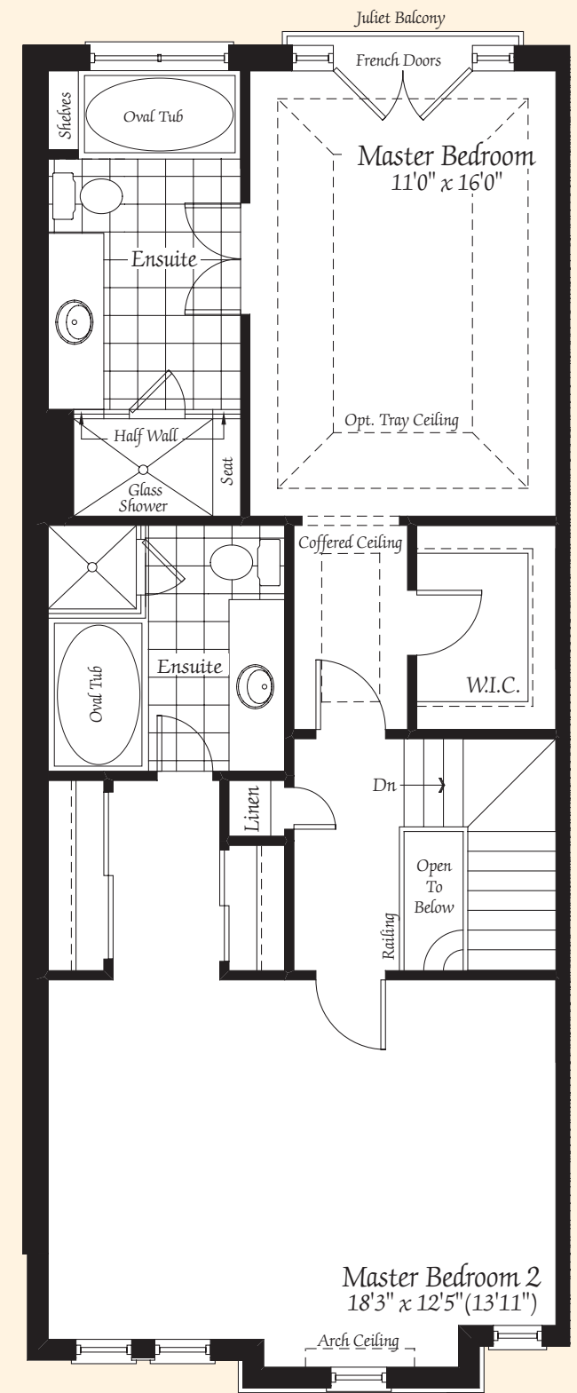
Optional Second Floor Elevation B
